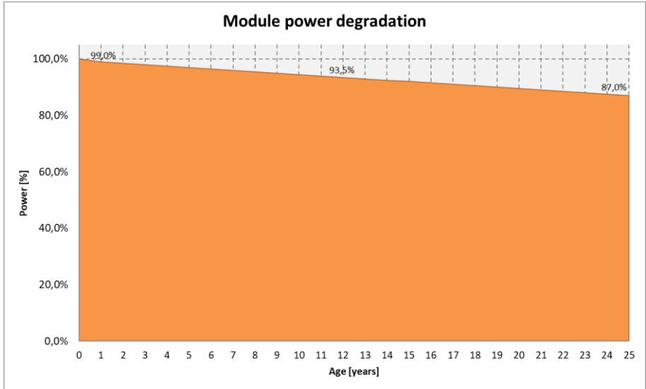
Picture 1. Power degradation graph
